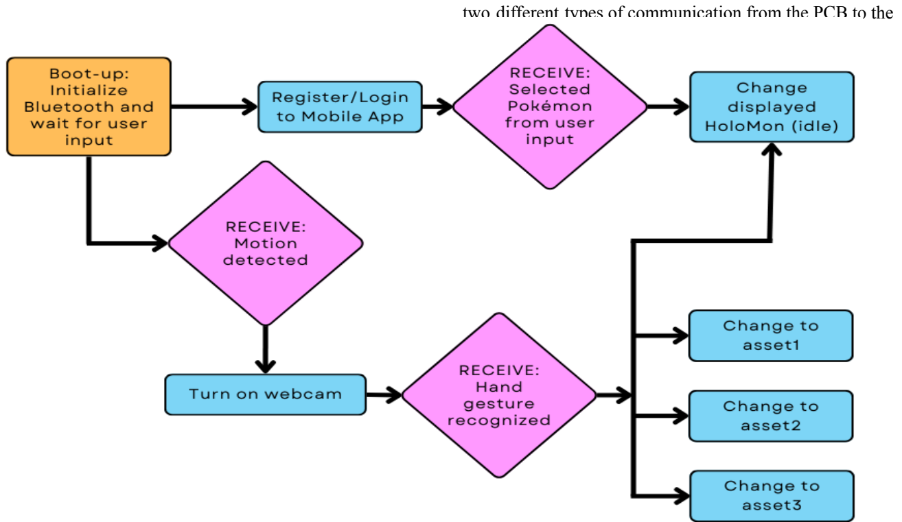
Figure 5. HoloMon data flow chart.
