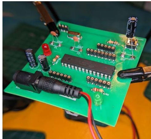
Figure 7. Soldered PCB.
